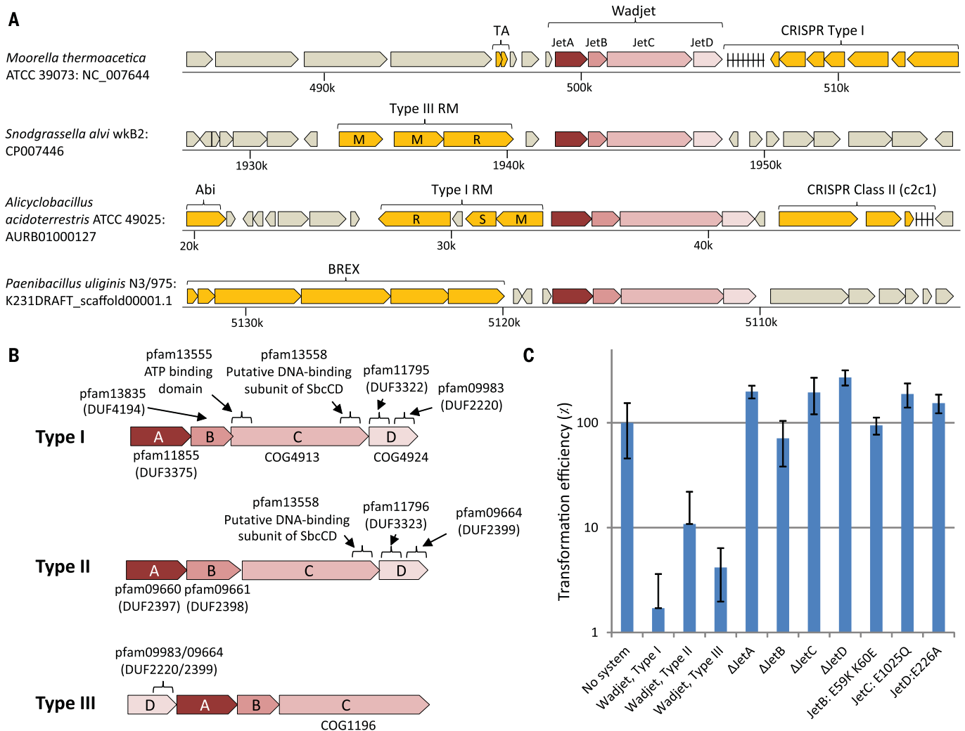
Fig. 5. The Wadjet system provides protection against plasmid transformation in B. subtilis . (A) Representative instances of the Wadjet system and their defense island context. Genes known to be involved in defense are orange. RM, restriction-modification; TA, toxin-antitoxin; Abi, abortive infection. (B) Domain organization of the three types of Wadjet. Pfam and COG domains were assigned according to the information in the IMG database (48). (C) Wadjet reduces plasmid transformation efficiency in B. subtilis . Instances
